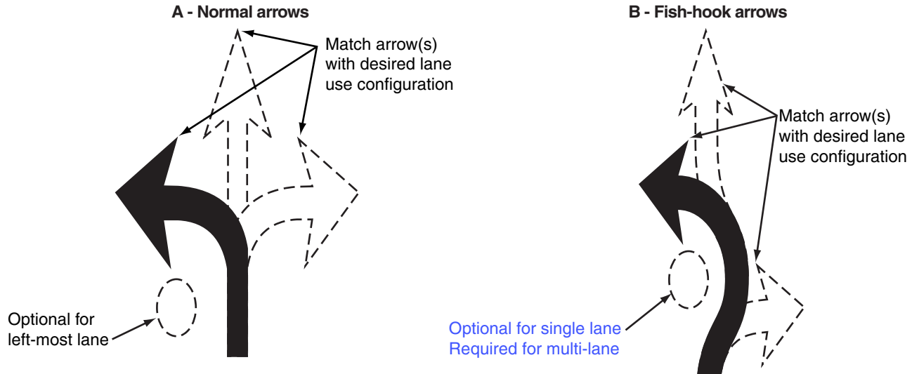
Figure 3C-2. Lane-Use Arrow Pavement Marking Options for Roundabout Approaches
