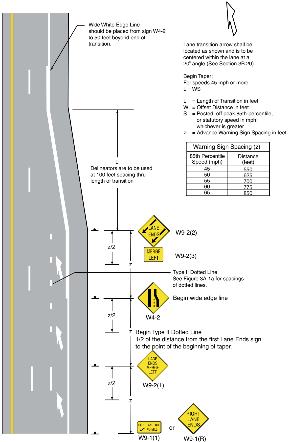
Figure 3B-14a. Examples of Lane Reduction Transition - Expressway
