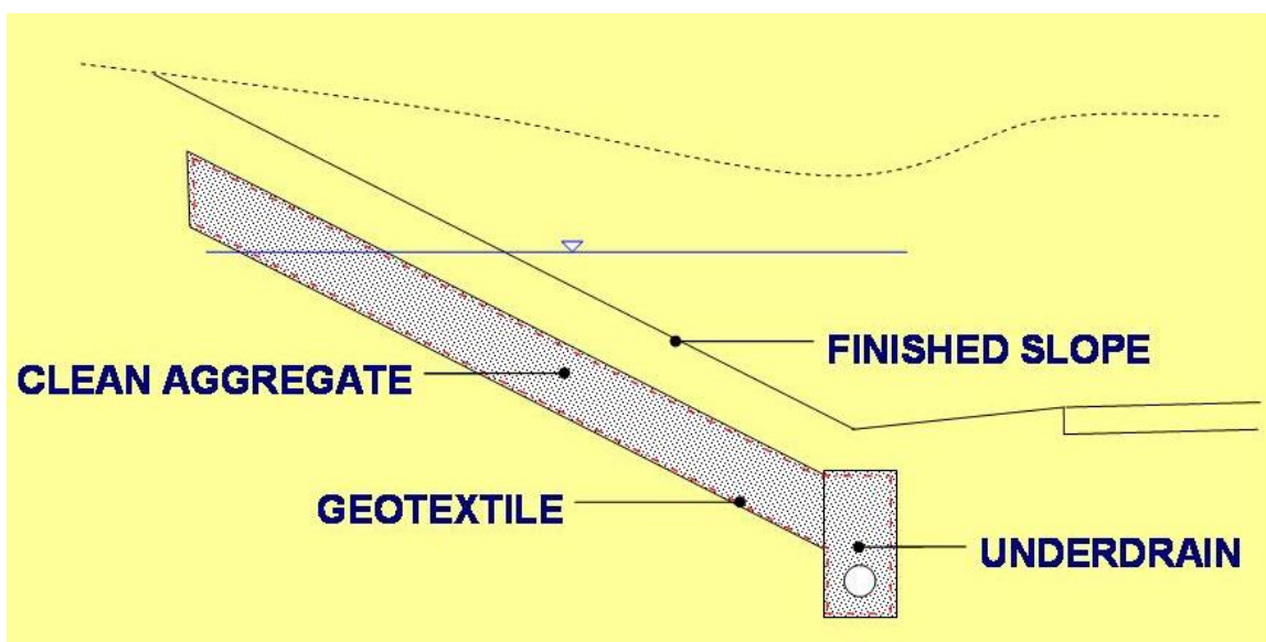
Slope Drainage Blanket Example – Cut Slope
