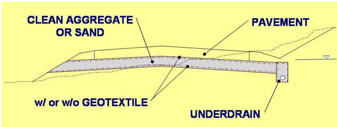
Drainage Blanket Example – Capping Layer
