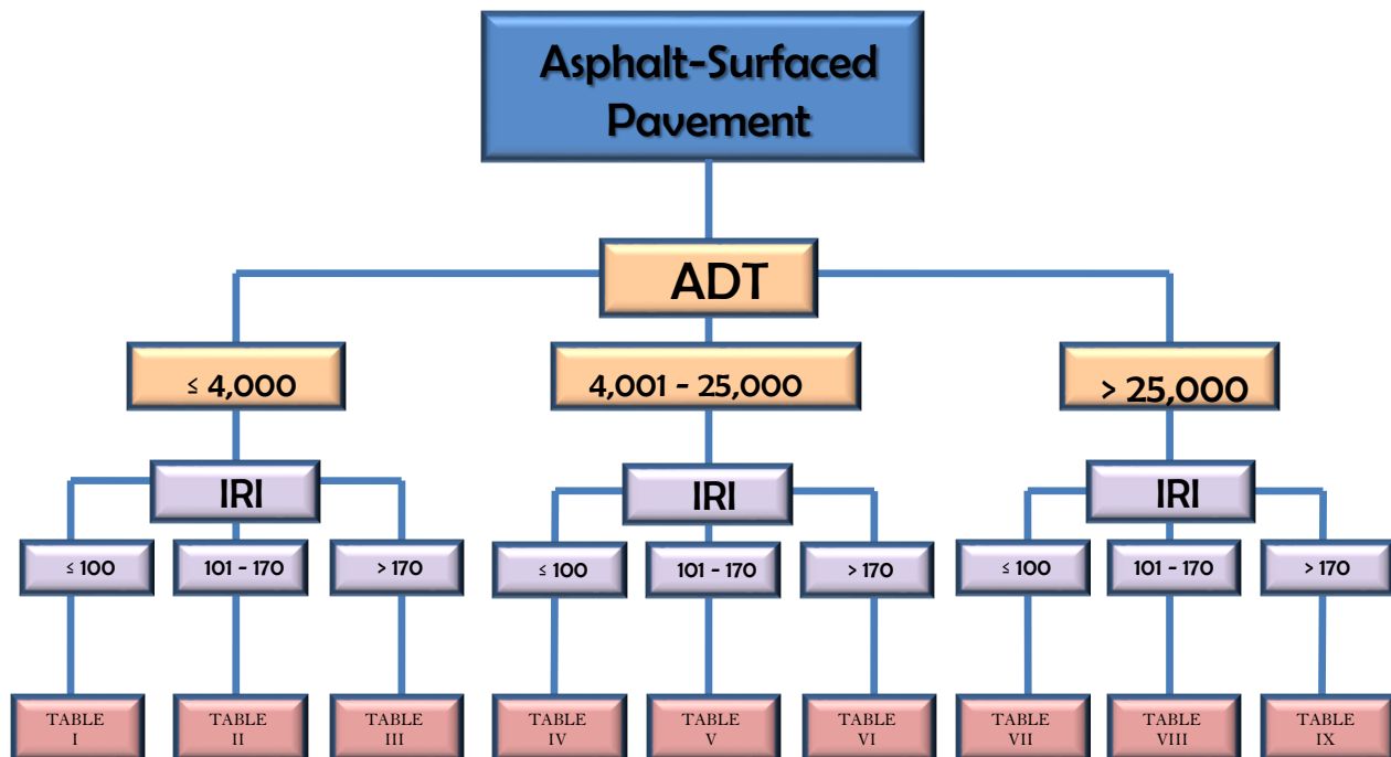
Figure 1 Decision Tree for Asphalt-Surfaced Pavements
