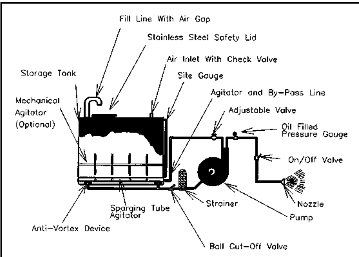
Drawing No. 3 Components of a Roadside Sprayer Side View
