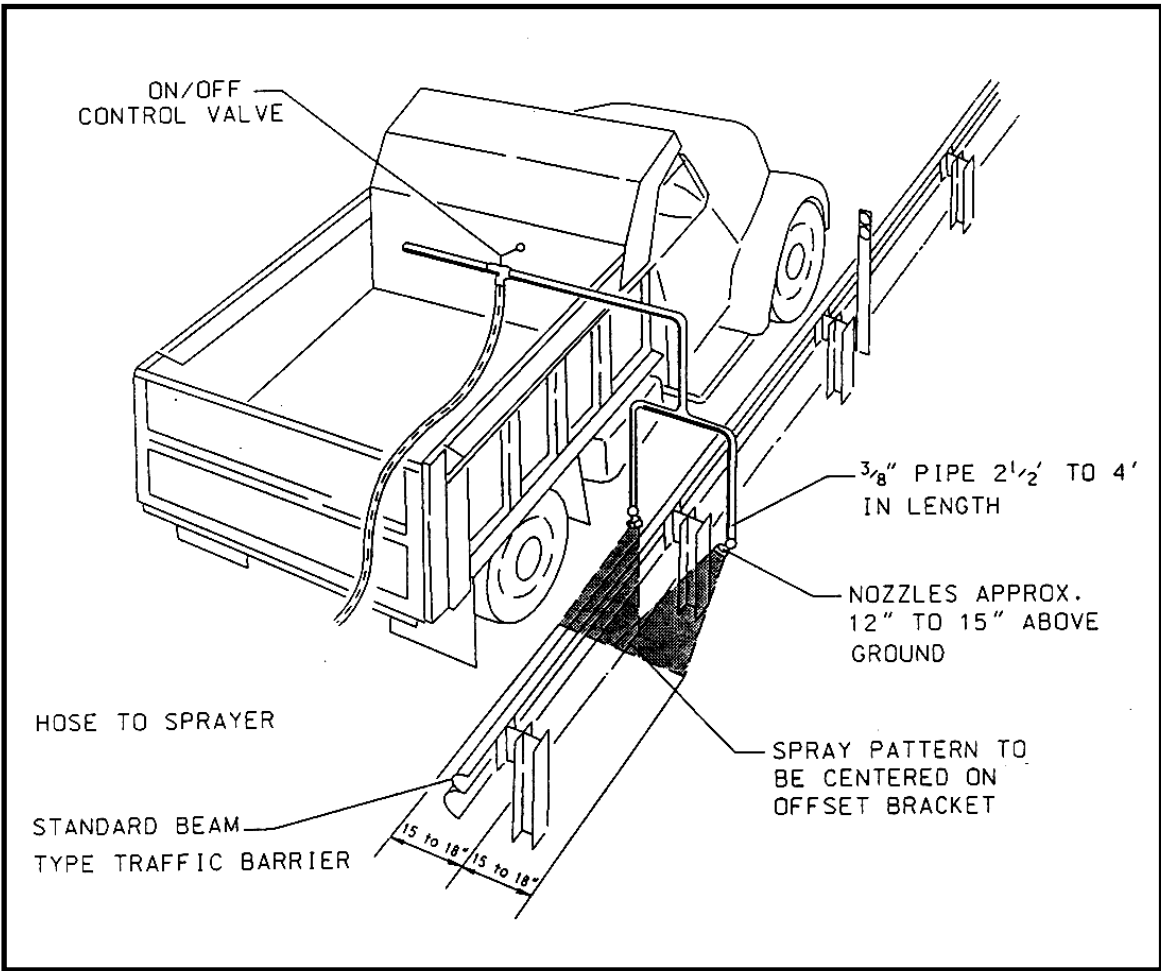
Drawing No. 4 Dual 1/4" 6510 or 6515 Nozzles Held Around Traffic Barrier
