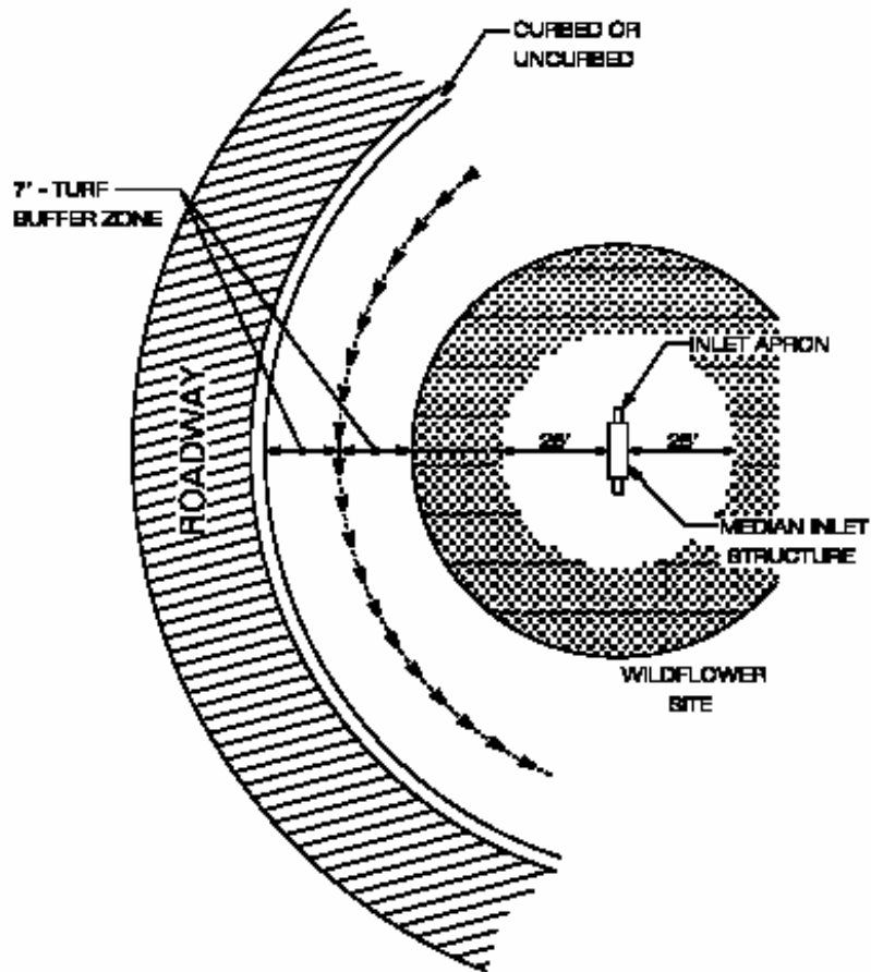
PLAN VIEW NO. 6 ROADSIDE RAMP - LESS THAN 4:1
