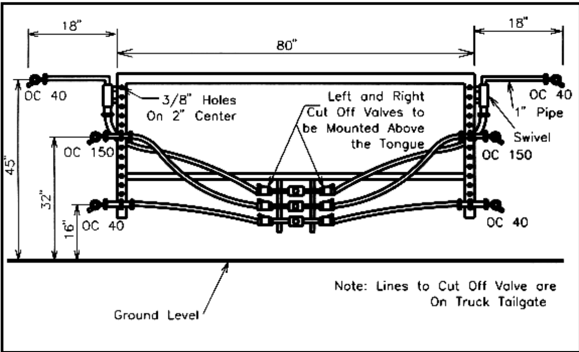
Drawing No. 2 Nozzle Arrangement 400 Gallon Roadside Herbicide Sprayer Front View
