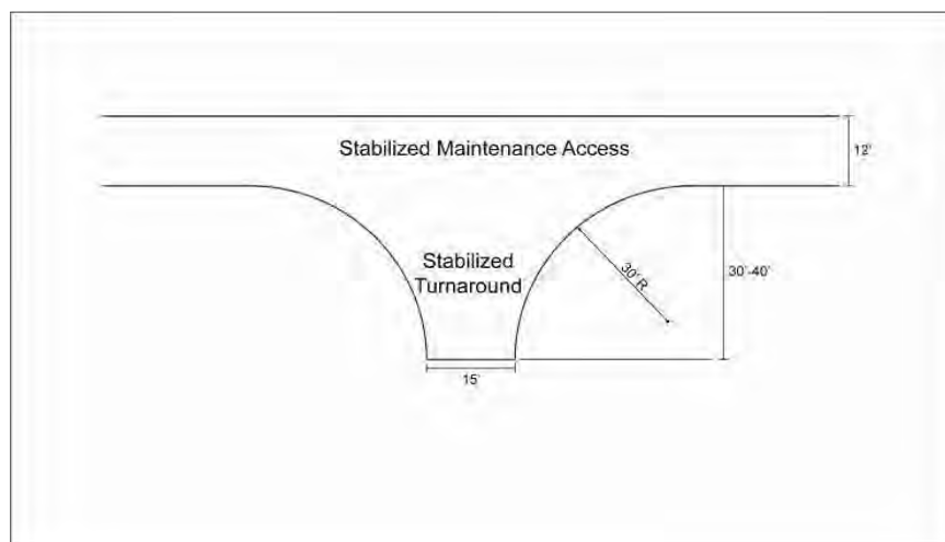
Figure 6-4. Turnaround Dimensions for Maintenance Vehicles
