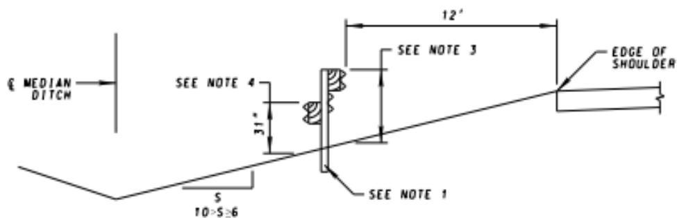
SECTION C-C END OF TRANSITION AT 12' OFFSET
