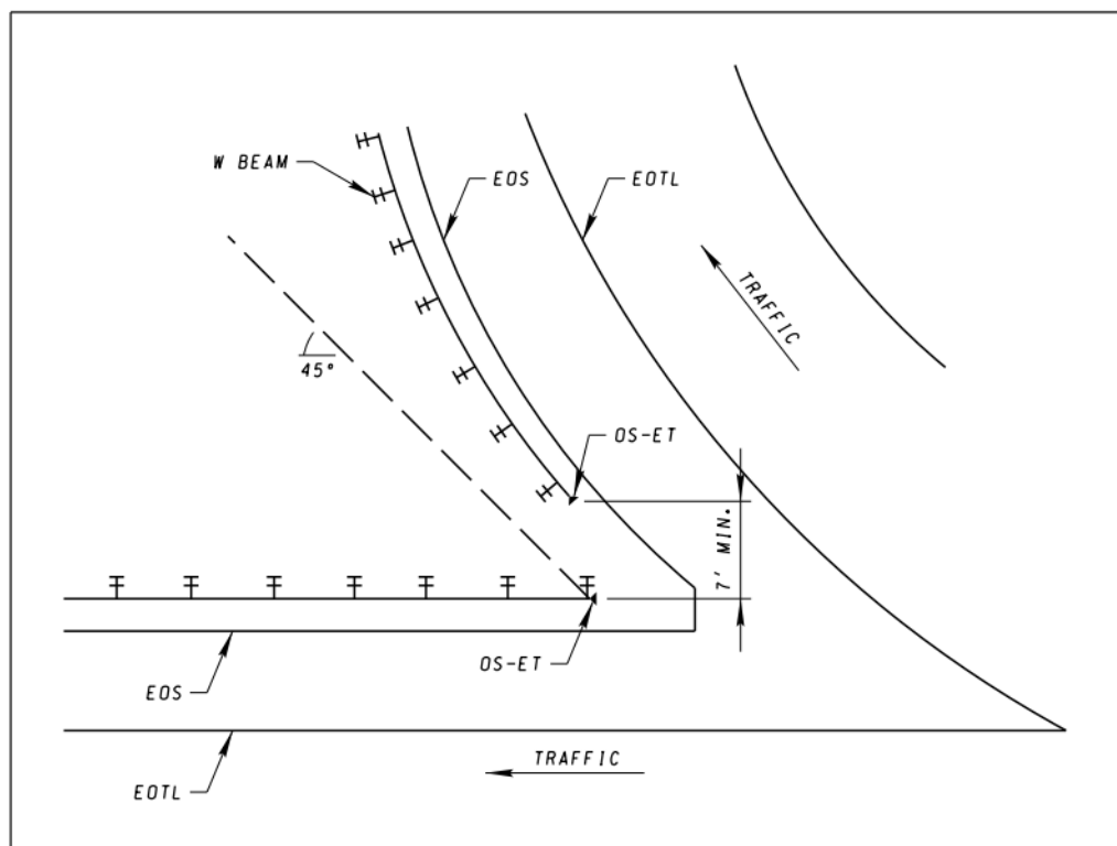
Figure 16: Gore End Treatment – OS-ET
