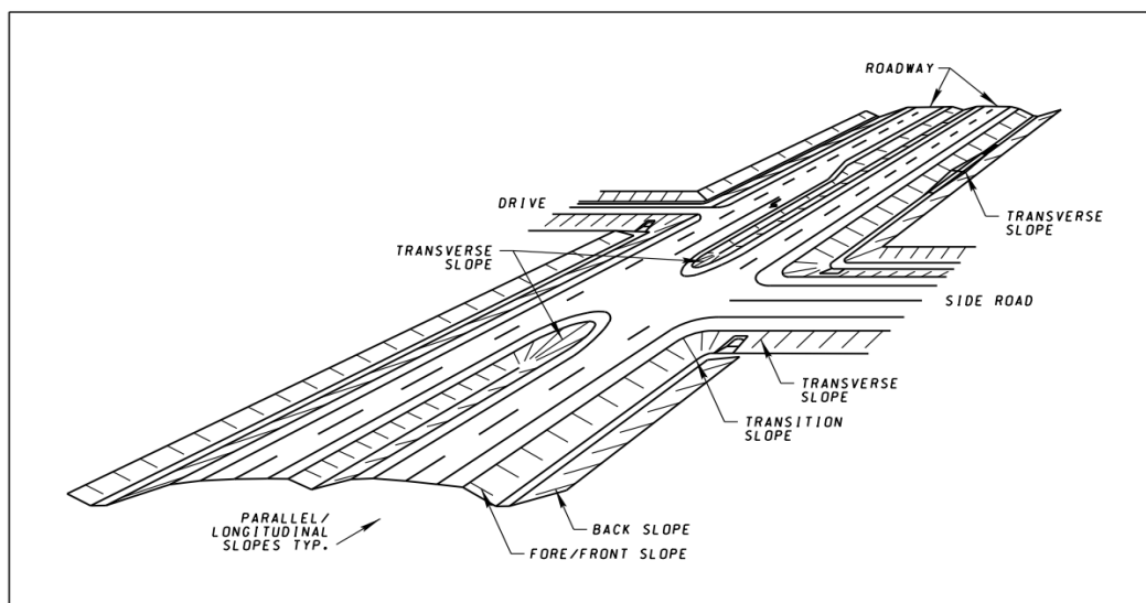
Figure 1: Roadside Slopes (Adapted from Figure 3-1 of the RDG) Source: AASHTO Roadside Design Guide, 4 th Edition
