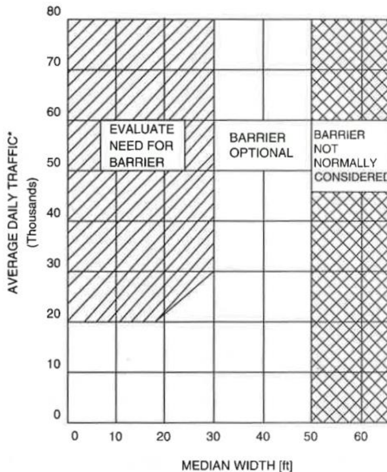
Figure 4: Guidelines for Median Barrier on High Speed, Fully Controlled-Access Roadways (Figure 6-1 of the RDG)
