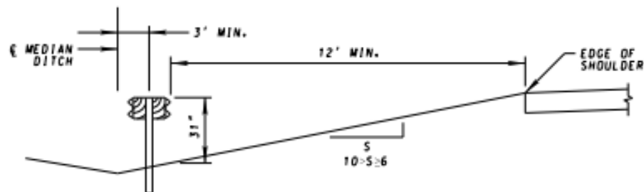
SECTION E-E NORMAL TBWB-MB AT 12' OR GREATER OFFSET
