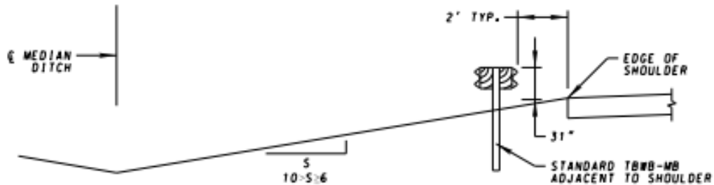
SECTION A-A STANDARD TBWB-MB AT 2' OFFSET
