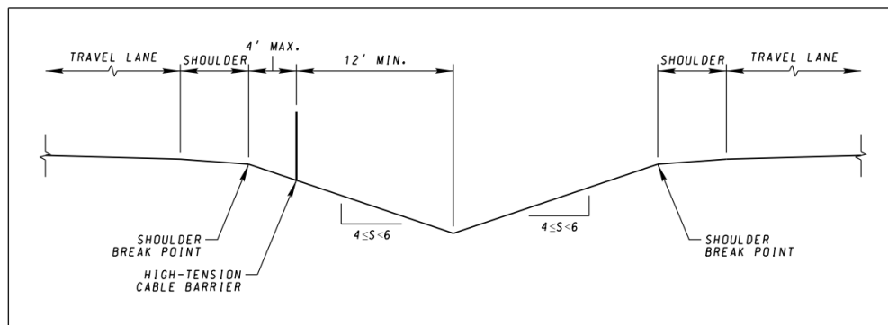
Figure 5: High-Tension Cable Barrier Placement on Slopes of 6:1 to 4:1
