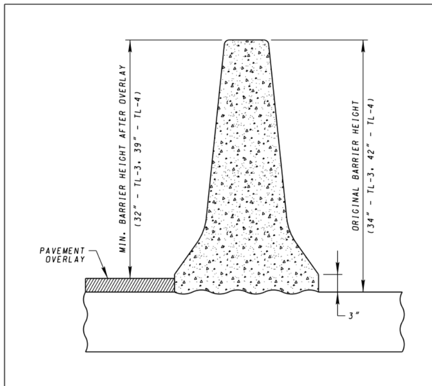
Figure 17: Pavement Resurfacing Considerations for Concrete Barrier
