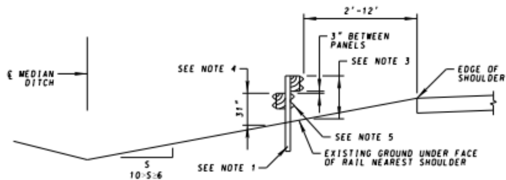
SECTION B-B TRANSITION ZONE - 2' TO 12' OFFSET
