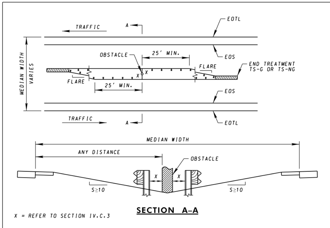
Figure 9: Example: Median, Flat Side Slope, Isolated Obstacle Inside Design Clear Zone of Both Roadways
