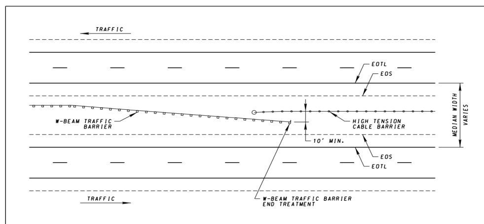
Figure 6: High-Tension Cable Barrier/W-Beam Traffic Barrier Transition Layout
