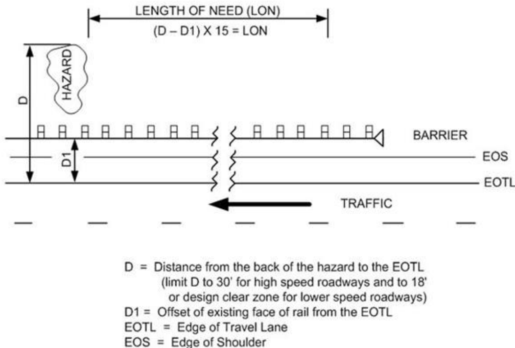
Figure 3: Field Expedient Approximation for LON (from W-Beam Guardrail Repair, FHWA, Nov. 2008)
