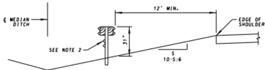
SECTION D-D TBWB-MB AT THE END OF HEIGHT TRANSITION
