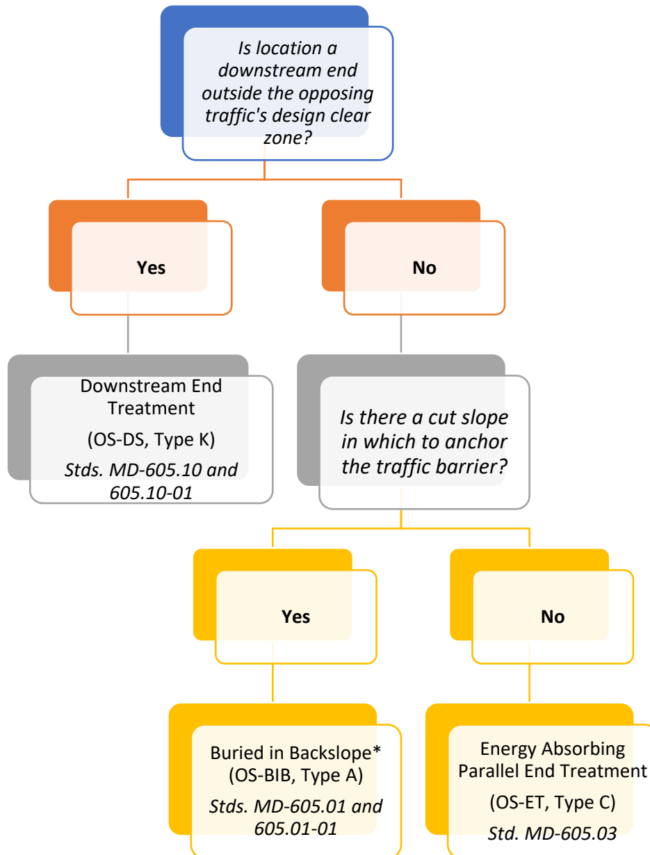
Flow Chart 1: Roadside End Treatment Selection Guidance
