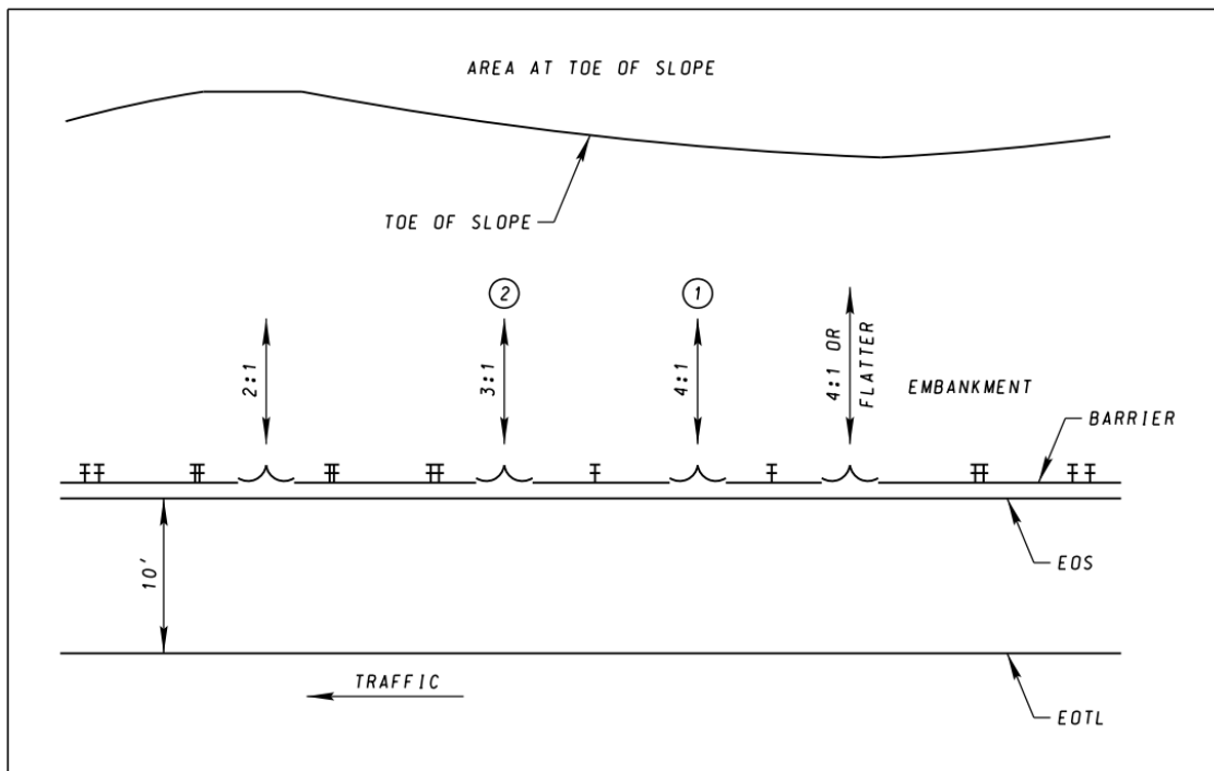
Figure 7: Example: Critical Embankment
