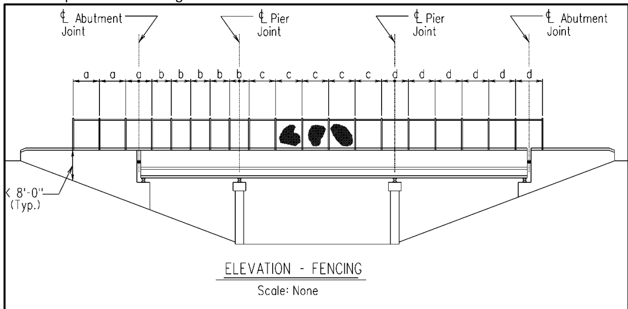
Figure 2-6: Fence Spacing on Bridges
