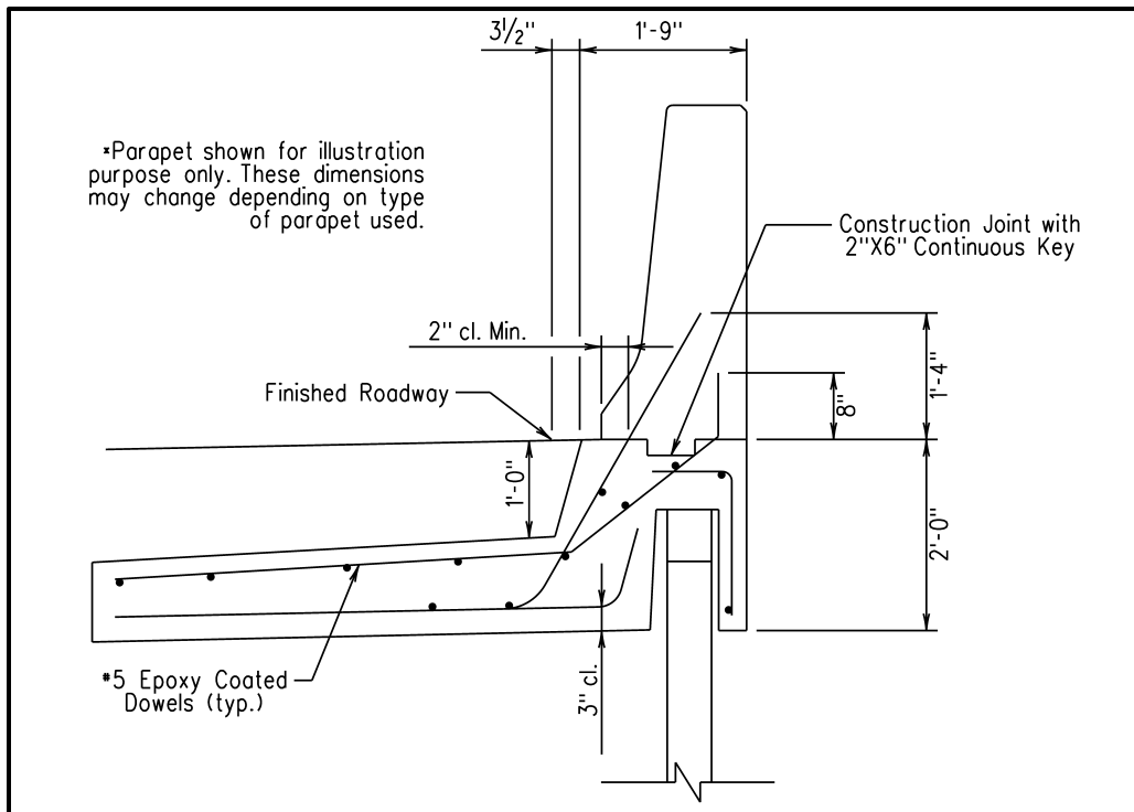
Figure 2-8: Barrier Doweled into Moment Slab
