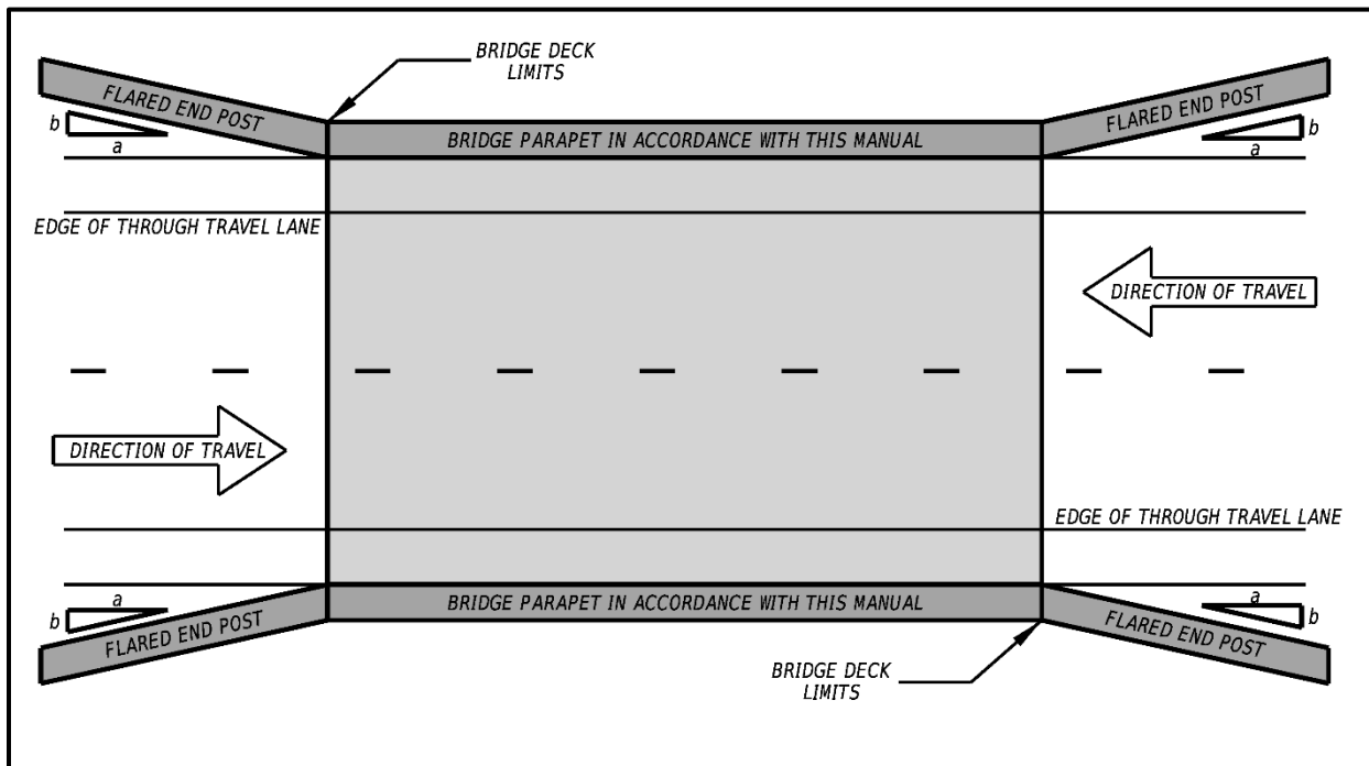
Figure 2-4: Tapered End Posts at Locations where Aesthetics is a concern and there is no Adjacent Guardrail
