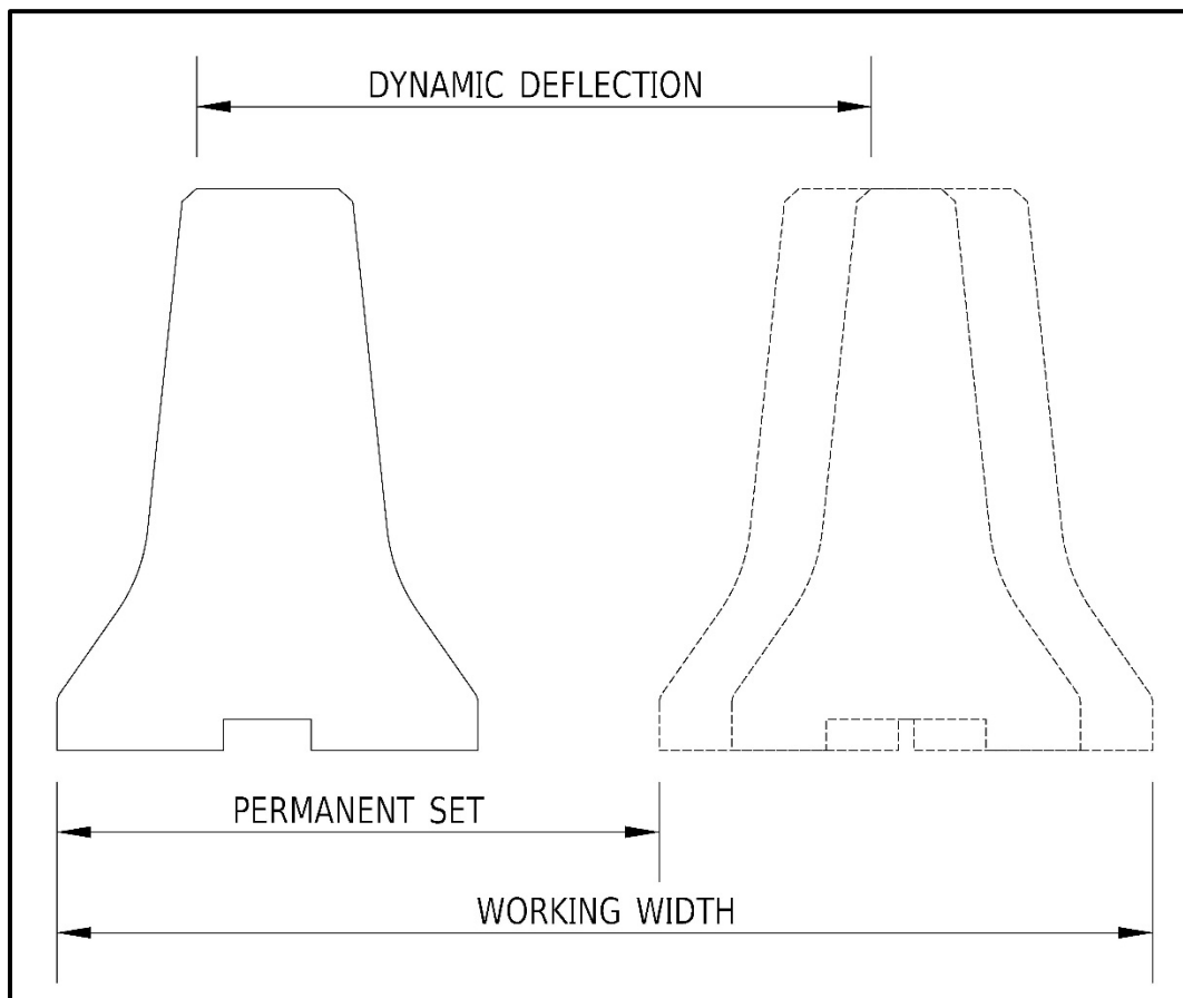
Figure 4-1: Barrier Deflection
