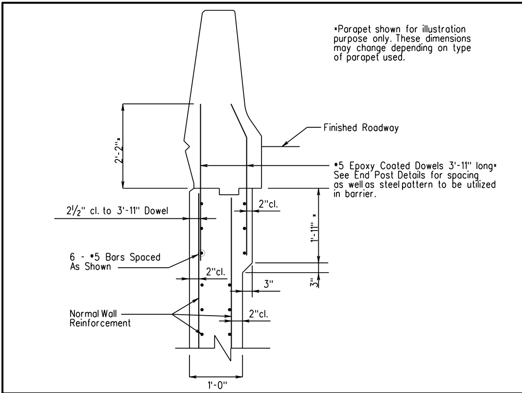
Figure 2-7: Parapet Attachment for Walls with 1'-0" Stem Thickness
