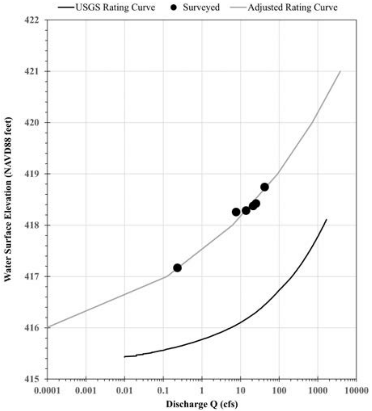
Figure 6. Upstream station (Site 01636845) rating curve
