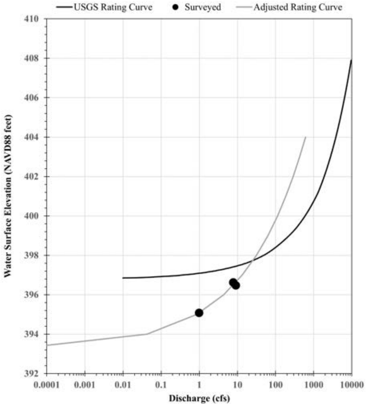
Figure 7. Downstream station (Site 01636846) rating curve
